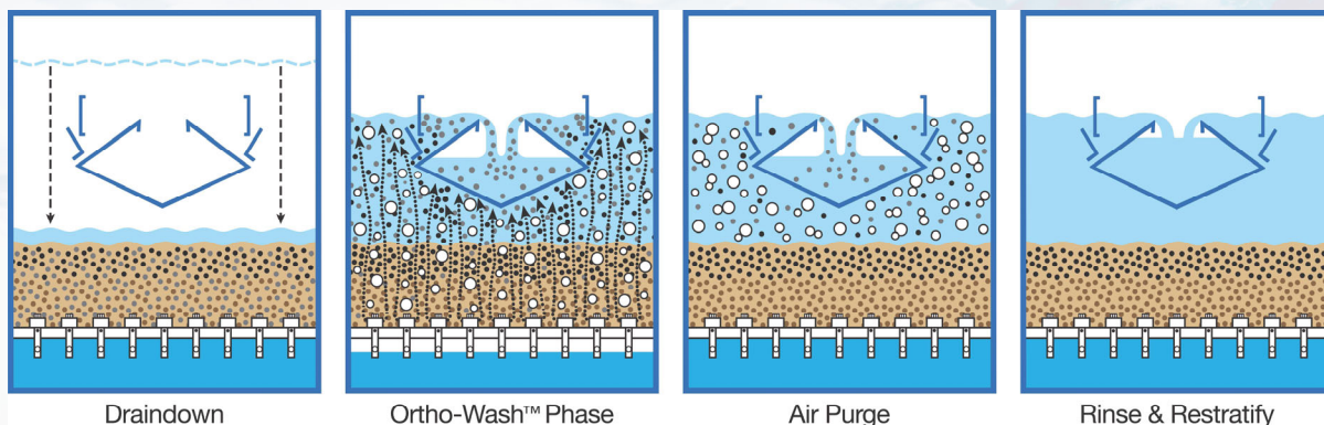
Ortho-Wash™ Simultaneous Backwash and Air Scour Process
