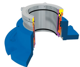
Double Mechanical Cartridge ChemSeal
