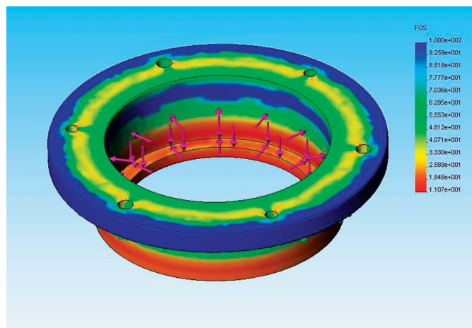
Example of FEA analysis
