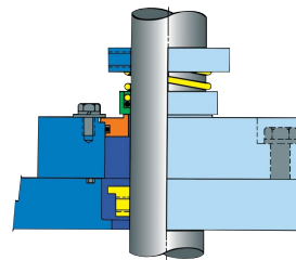
Single Mechanical Seal
